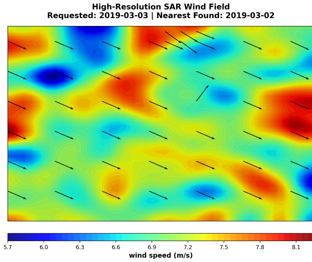
Figure 2: First visualization of the SAR predicted wind vector field utilizing the deployed API.
